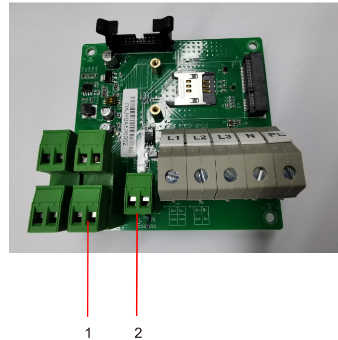
Wiring definition in the side window
